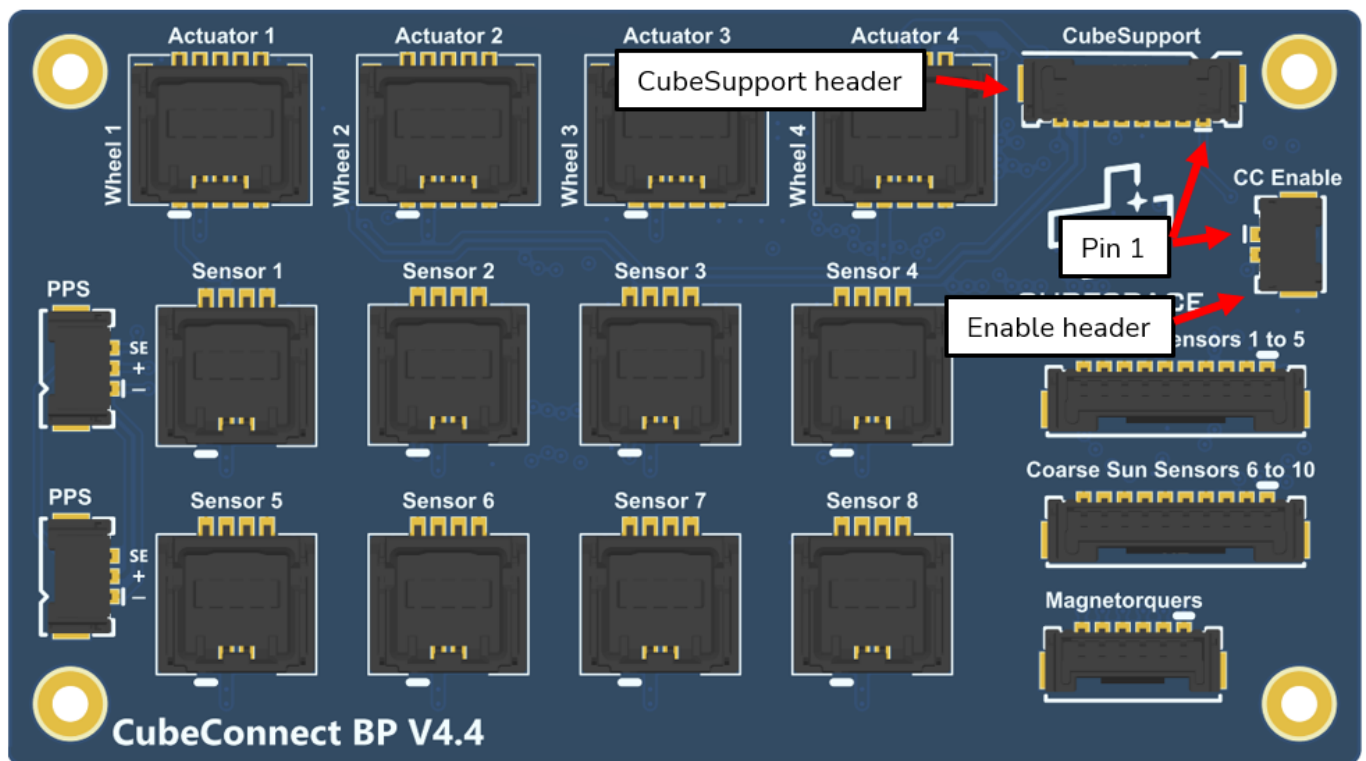
Figure 33: CubeConnect PCB (Backplane Variant) – Ground Support Headers
