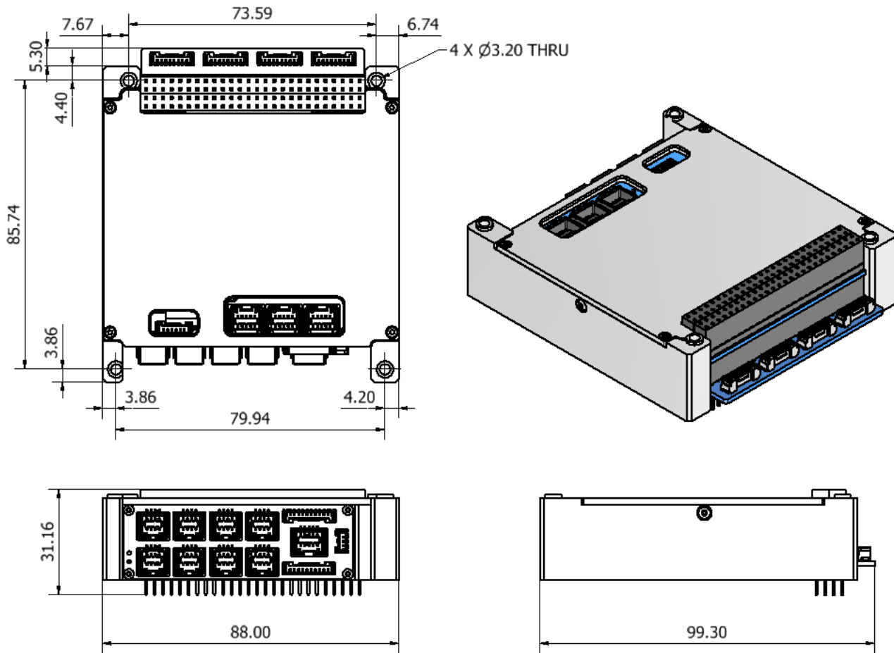
Figure 50: Indicative Dimensions of CubeADCS Core PC104 with the Midstack-Mount V_{\text{Bat}} Bypass CubeDoor PCB with Upward-facing Headers
