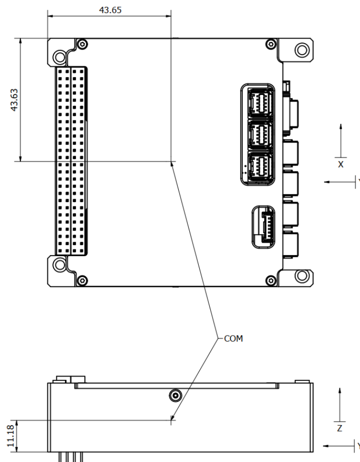
Figure 36: CoM Position of the Standard PC104 CubeADCS Core
