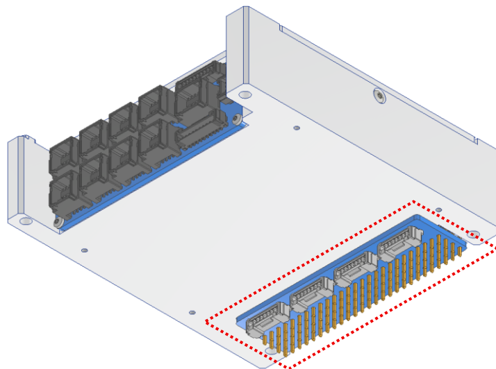
Figure 7: V_{Bat} Bypass Bottom-Mount variant for CubeADCS Core PC104
