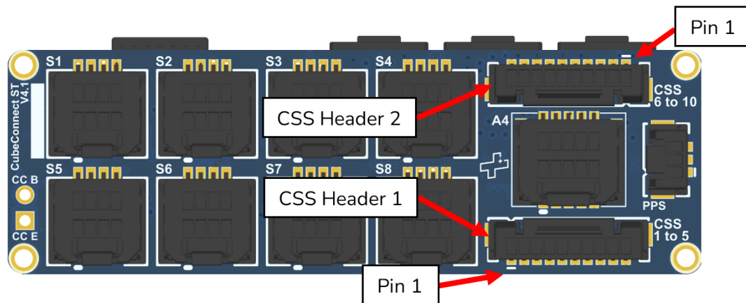
Figure 28: CubeConnect PCB (PC104 Variants) – Coarse Sun Sensors Headers
