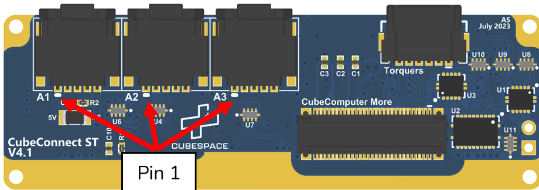
Figure 24: CubeConnect (PC104 Variants) – Pin 1 Indicated for Actuators 1-3
