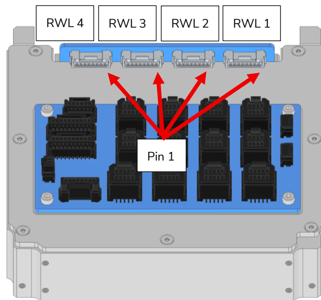
Figure 57: V_{Bat} Bypass PCB, Reaction Wheel Headers (Backplane Variant)
