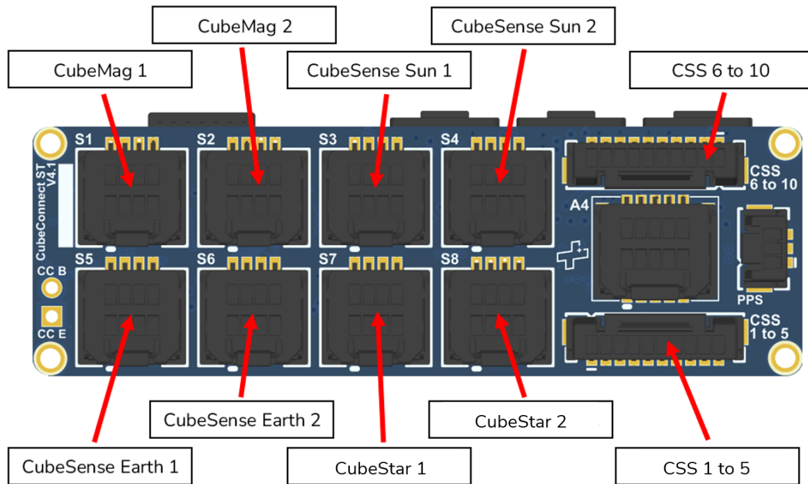
Figure 19: Example Configuration of External Sensors Connected to a PC104 Variant of CubeConnect
