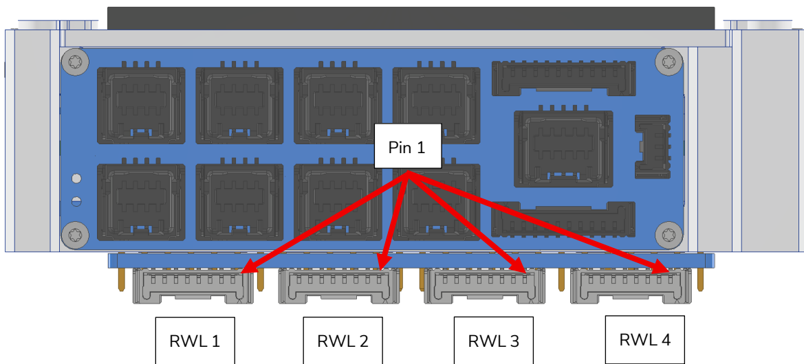
Figure 54: V_{\text{Bat}} Bypass PCB, Reaction Wheel Headers (PC104, Bottom-Mount Variant)
