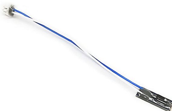
Figure 45: Single Coarse Sun Sensor PCB and Wire Harness
