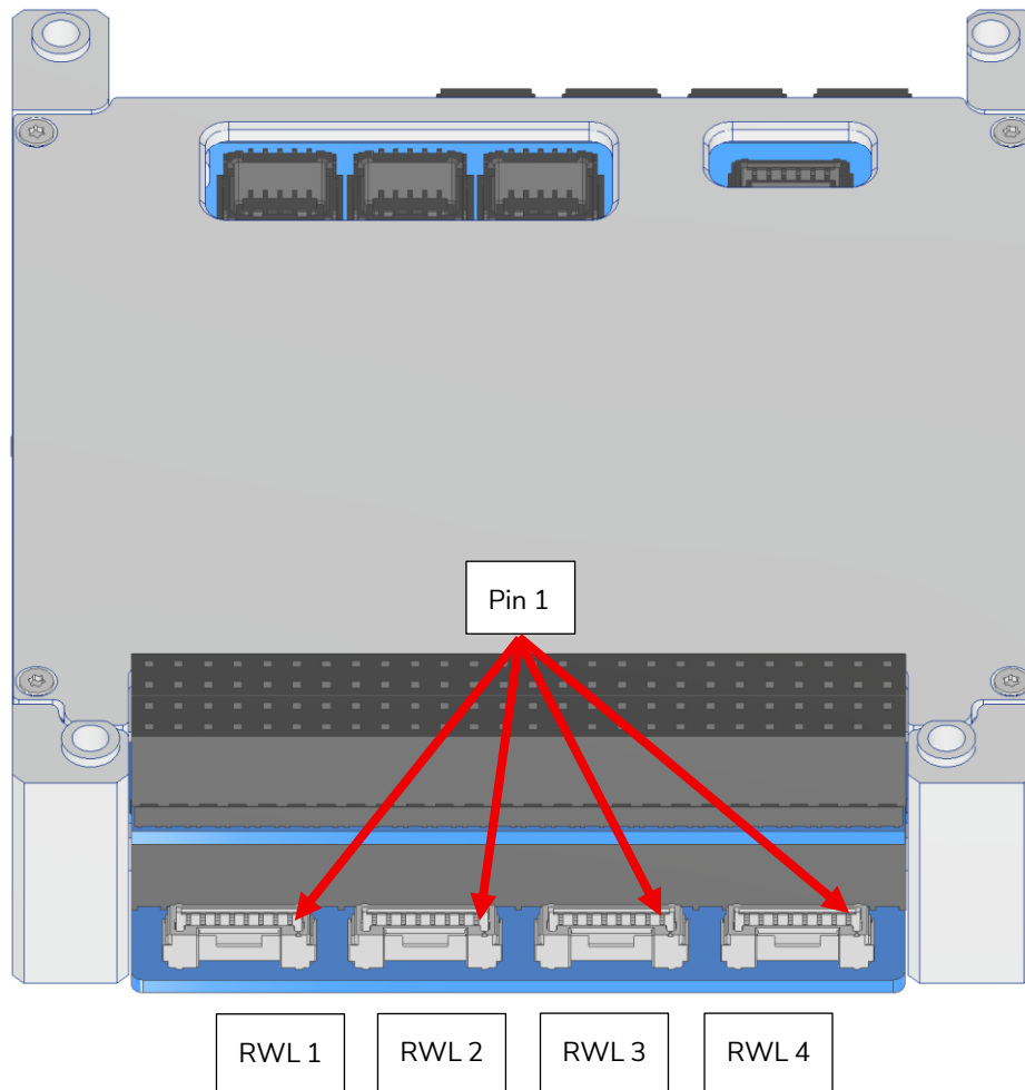
Figure 55: V_{Bat} Bypass PCB, Reaction Wheel Headers (PC104, Midstack-Mount Upward-Facing Headers Variant) – Top View
