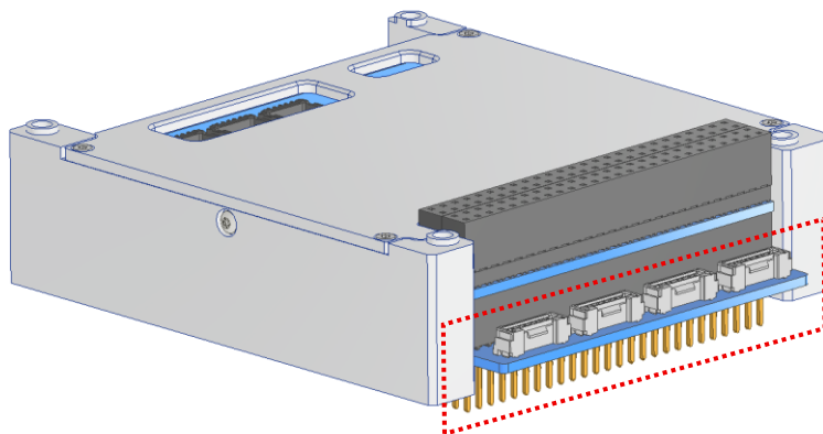
Figure 8: V_{Bat} Bypass Midstack-Mount variant (upward-facing headers) for CubeADCS Core PC104
