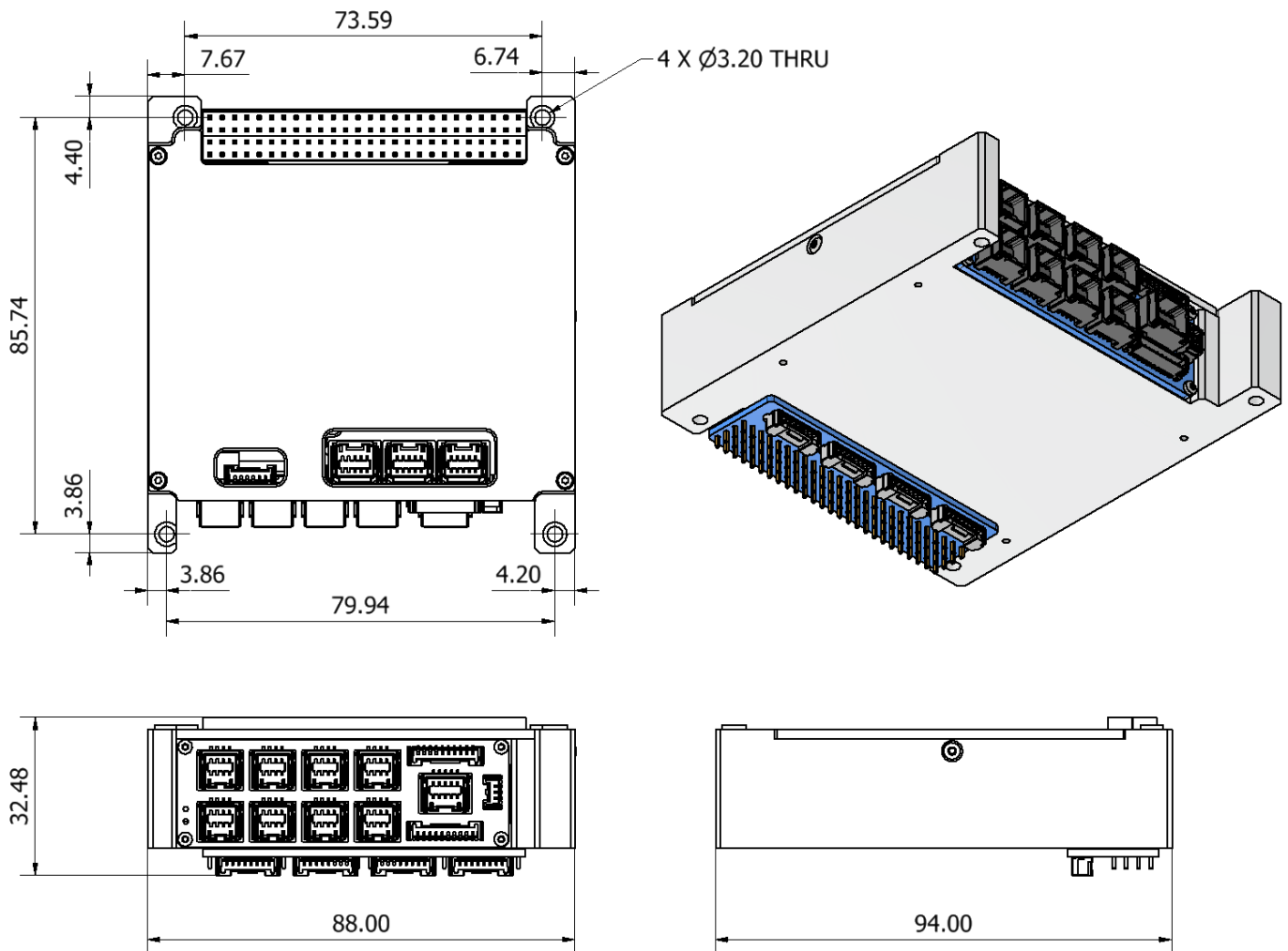
Figure 49: Indicative Dimensions of CubeADCS Core PC104 with the Bottom-Mount V_{Bat} Bypass CubeDoor PCB
