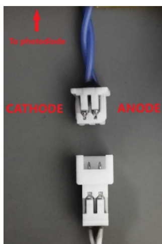
Figure 46: Coarse Sun Sensor In-line Harness Pins
