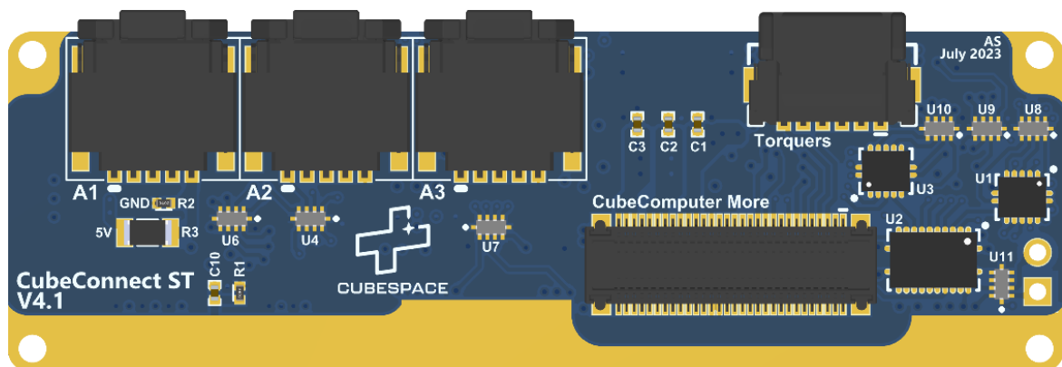
Figure 17: CubeConnect PCB (PC104 Variants) – Interior (Back) View
