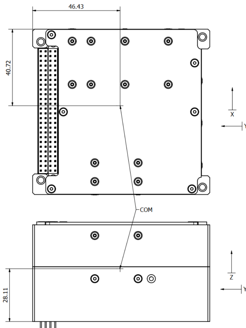
Figure 38: CoM Position of the PC104 CubeADCS Core Stack for 3U Satellites
