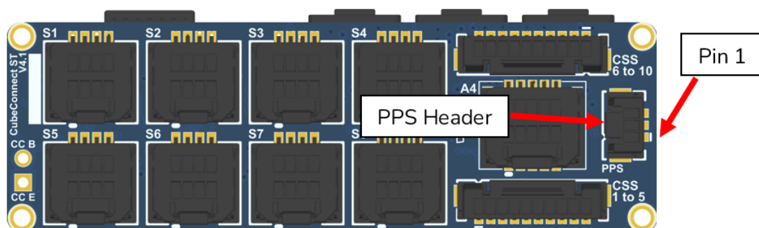
Figure 30: CubeConnect PCB (PC104 Variants) – PPS Header
