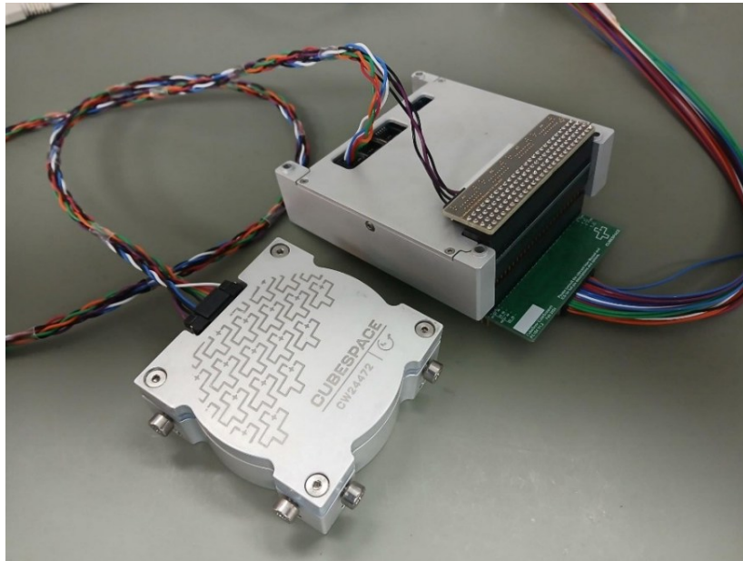
Figure 58: Single CW0500 reaction wheel plugged into CubeADCS Core PC104 with a Top-Mount V_{\text{Bat}} Bypass CubeDoor PCB
