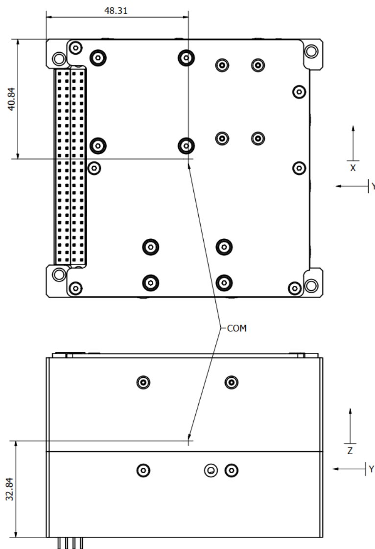
Figure 40: CoM Position of the PC104 CubeADCS Core Stack for 3U to 6U Satellites
