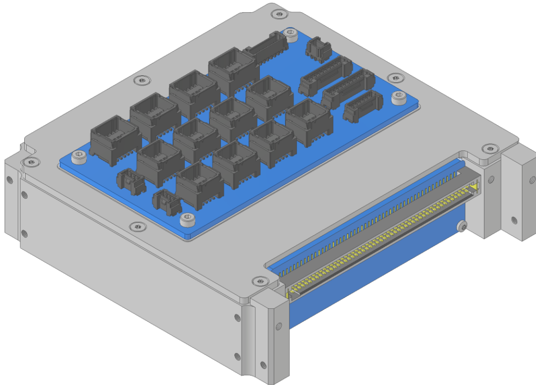
Figure 4: Backplane Variant of CubeADCS Core
