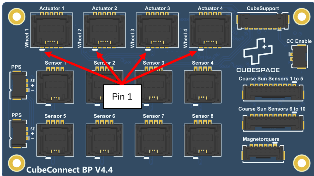
Figure 25: CubeConnect (Backplane Variant) - Pin 1 Indicated for Actuators 1-4
