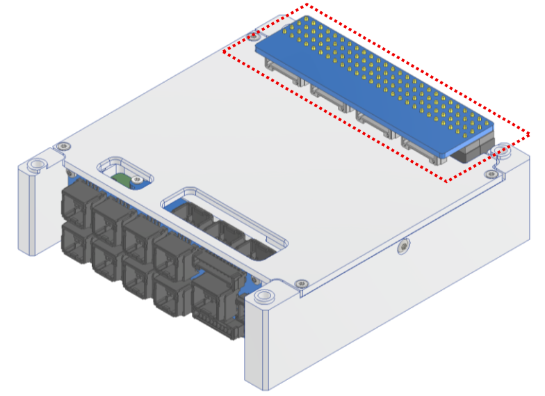
Figure 6: V_{Bat} Bypass Top-Mount variant for CubeADCS Core PC104
