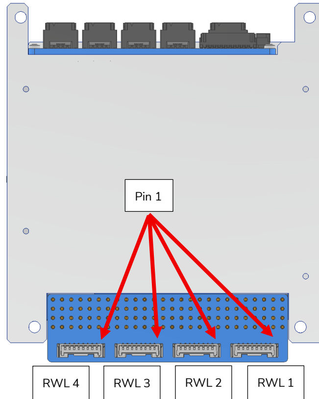
Figure 56: V_{Bat} Bypass PCB, Reaction Wheel Headers (PC104, Midstack-Mount Downward-Facing Headers Variant) – Bottom View
