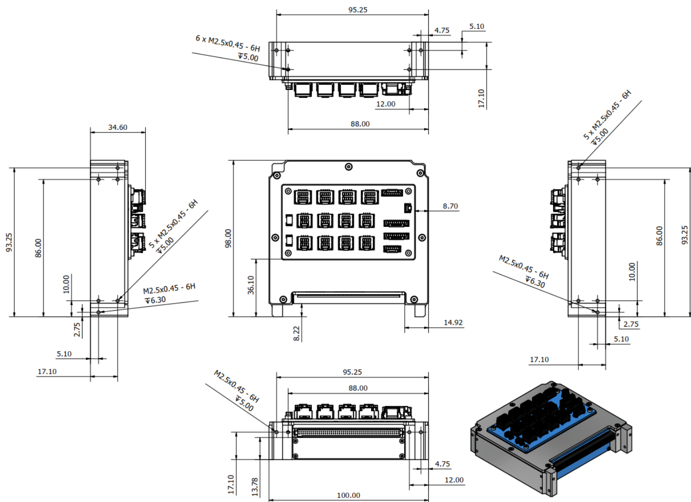
Figure 41: Indicative Dimensions of the Backplane CubeADCS Core
