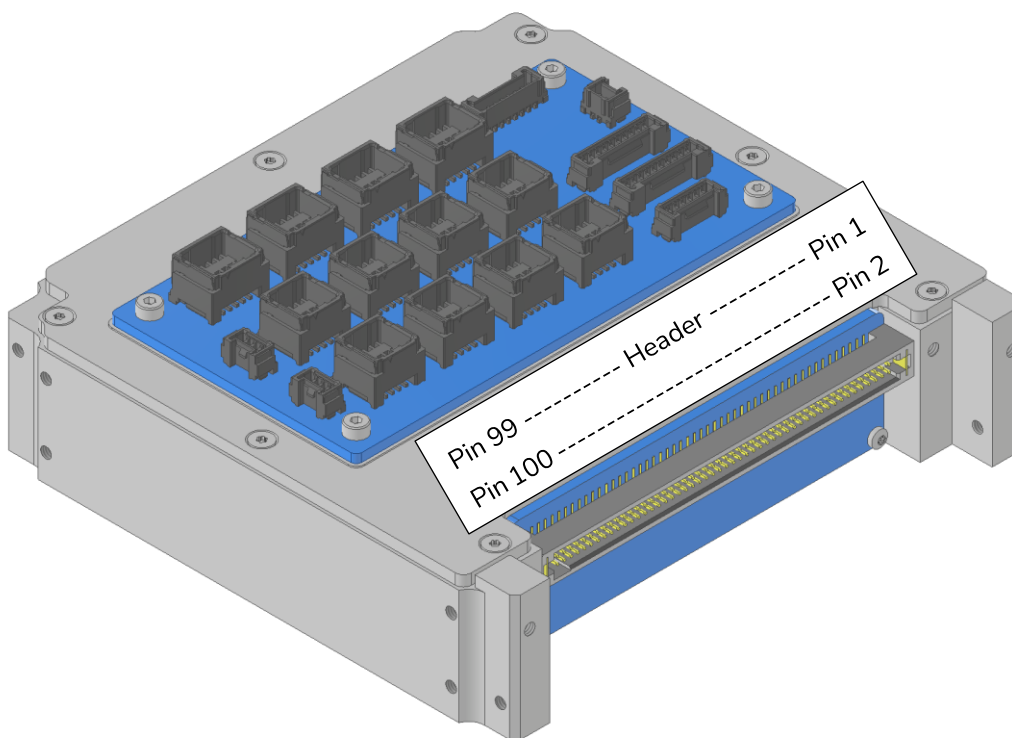
Figure 15: CubeADCS Core, Backplane Variant, Showing CubeDoor Header
