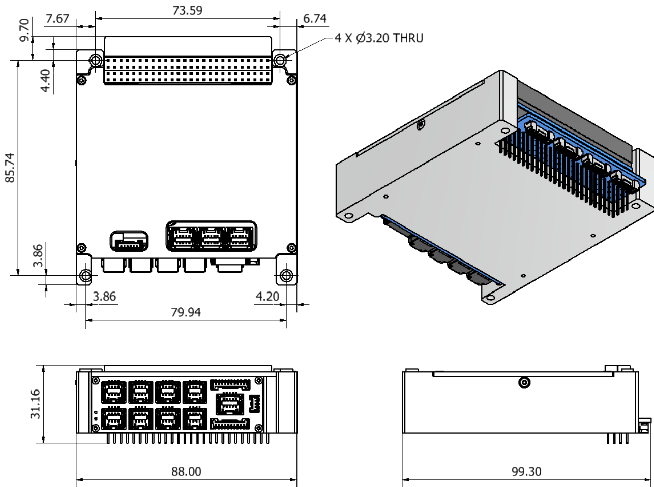
Figure 51: Indicative Dimensions of CubeADCS Core PC104 with the Midstack-Mount V_{\text{Bat}} Bypass CubeDoor PCB with Downward-facing Headers
