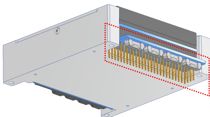
Figure 9: V_{Bat} Bypass Midstack-Mount variant (downward-facing headers) for CubeADCS Core PC104
