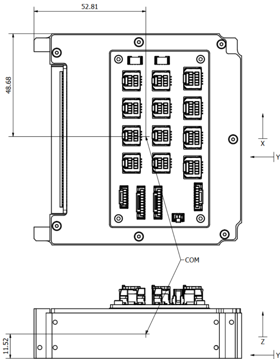
Figure 42: CoM Position of the Backplane CubeADCS Core
