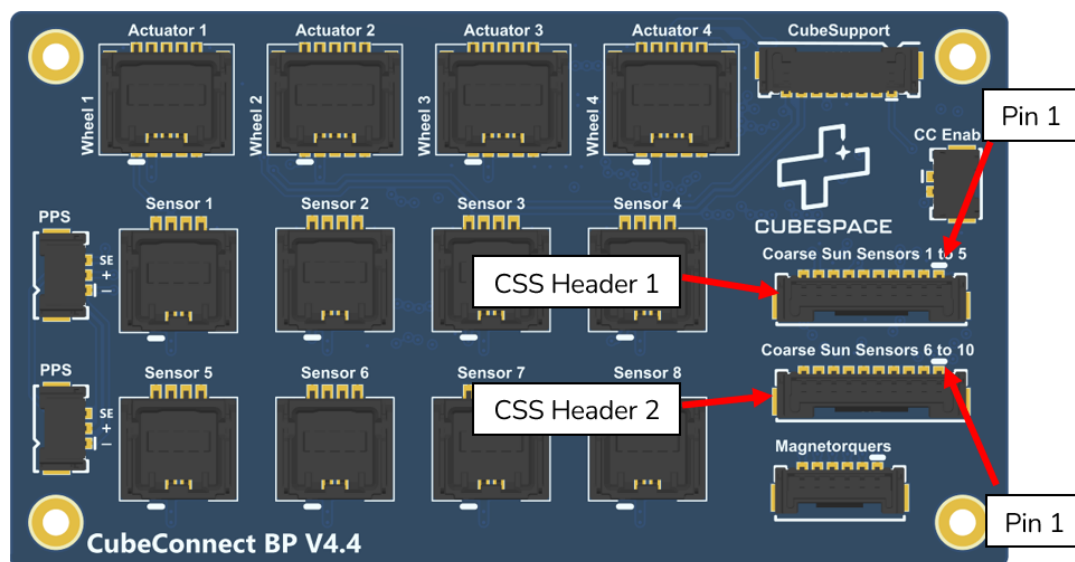
Figure 29: CubeConnect PCB (Backplane Variant) - Coarse Sun Sensors Headers
