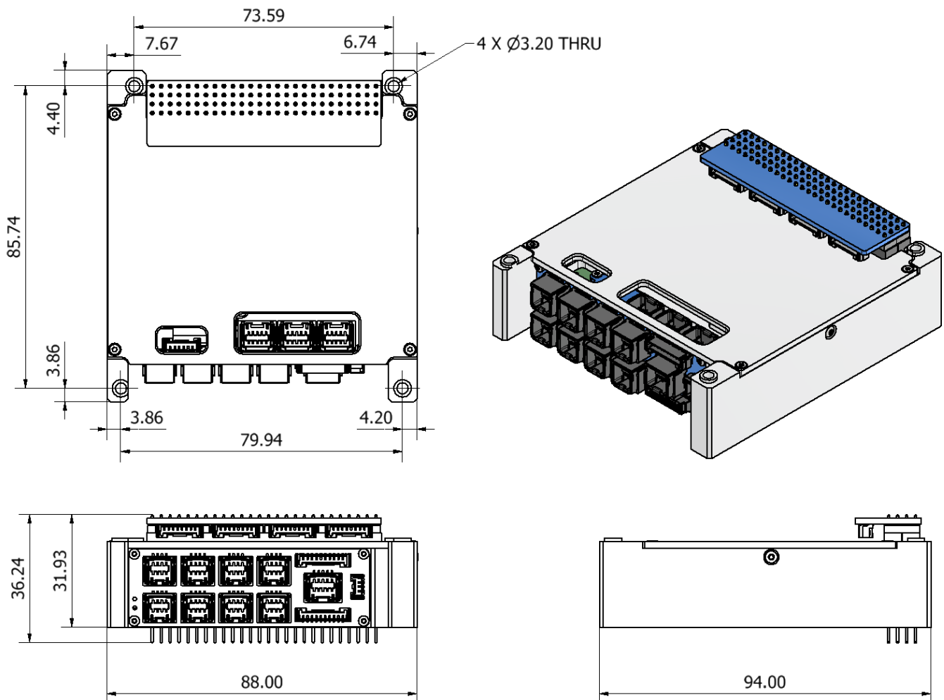
Figure 48: Indicative Dimensions of CubeADCS Core PC104 with the Top-Mount V_{\text{Bat}} Bypass CubeDoor PCB
