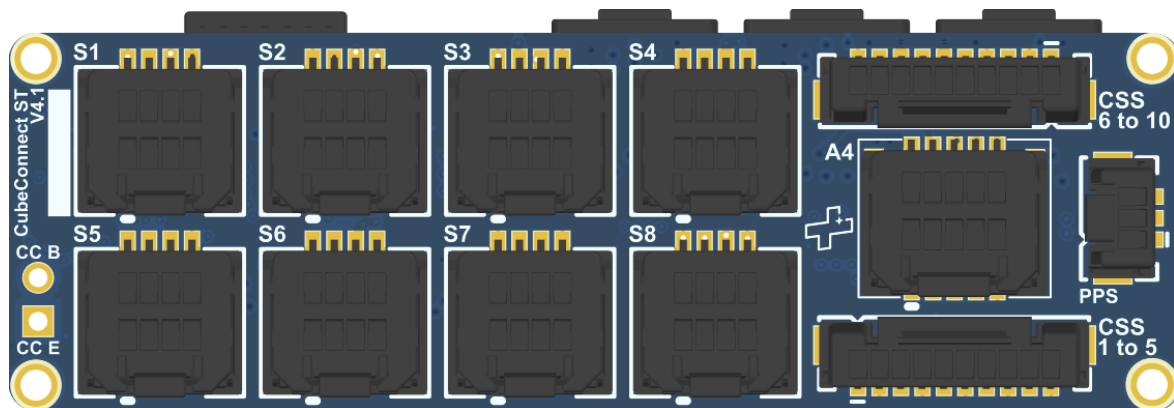
Figure 16: CubeConnect PCB (PC104 Variants) – Exterior (Front) View
