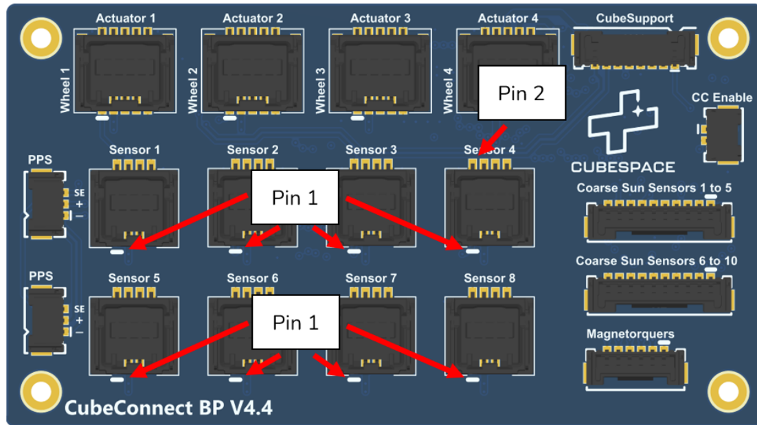
Figure 27: CubeConnect (Backplane Variant) - Pin 1 Indicated for Sensors 1-8
