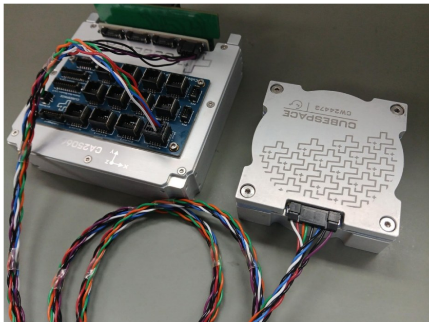
Figure 59: Single CW0500 reaction wheel plugged into CubeADCS Core Backplane with a V_{\text{Bat}} Bypass CubeDoor PCB
