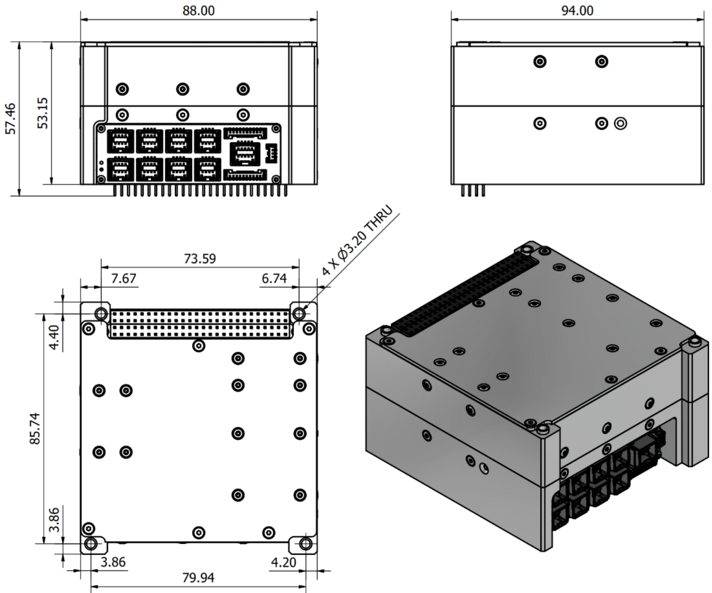
Figure 37: Indicative Dimensions of the PC104 CubeADCS Core Stack for 3U Satellites
