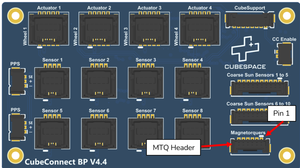
Figure 22: CubeConnect PCB, Backplane Variant - Magnetorquer Header
