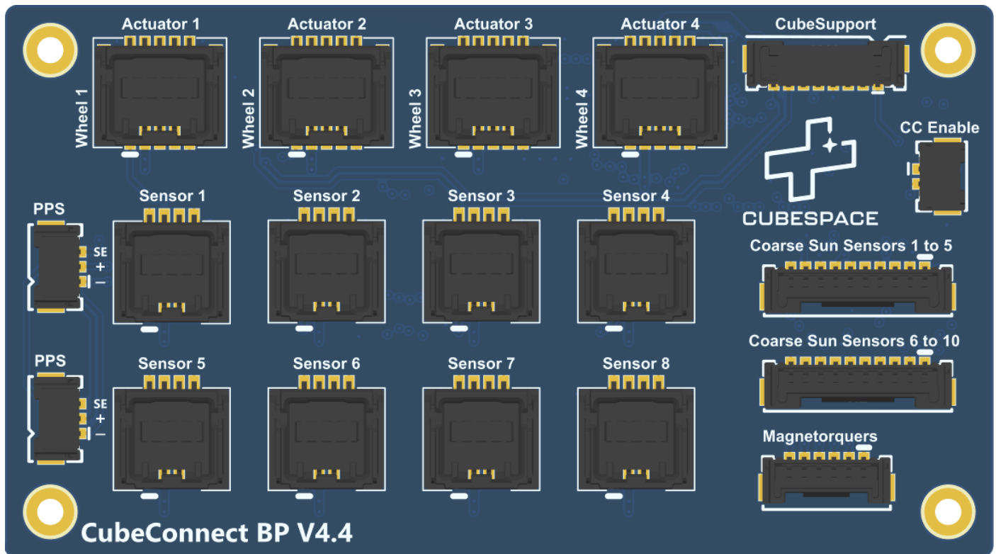
Figure 18: CubeConnect PCB (Backplane Variant) – Top View
