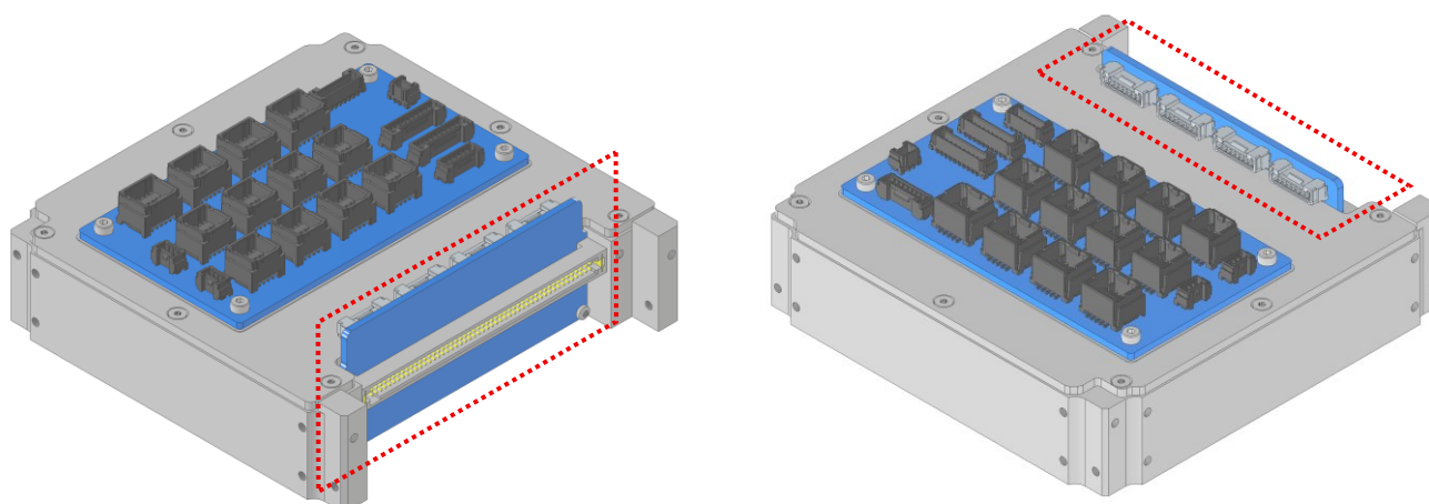
Figure 10: Two perspectives of the V_{Bat} Bypass option for CubeADCS Core Backplane
