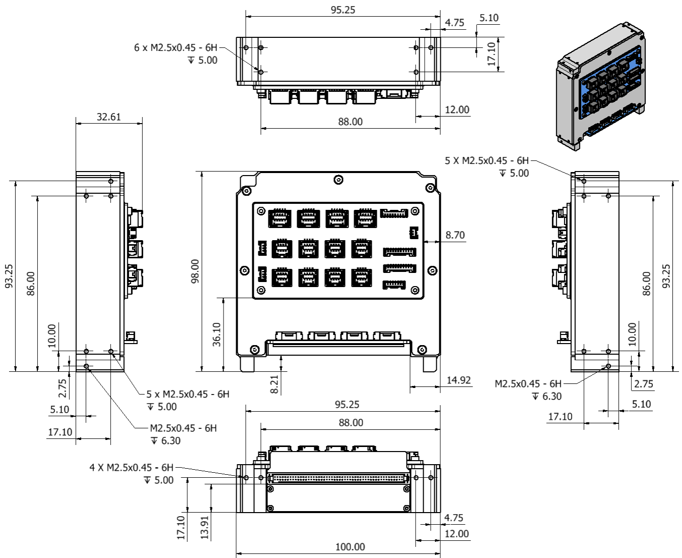
Figure 52: Indicative Dimensions of CubeADCS Core Backplane with the V Bat Bypass CubeDoor PCB
