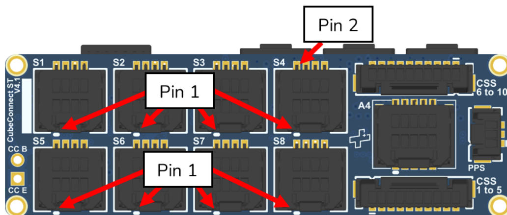
Figure 26: CubeConnect (PC104 Variants) - Pin 1 Indicated for Sensors 1-8
