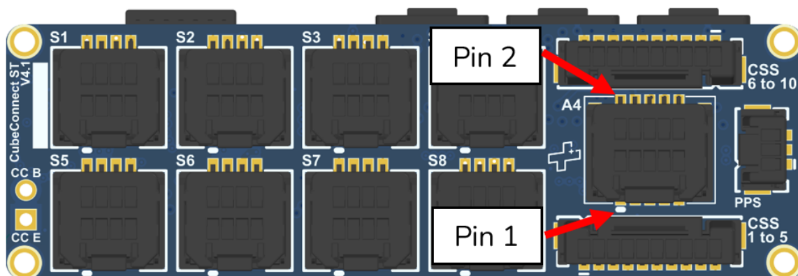
Figure 23: CubeConnect (PC104 Variants) – Pin 1 Indicated for Actuator 4
