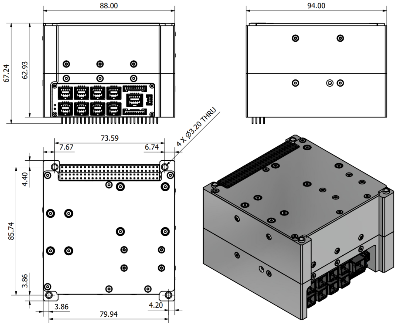
Figure 39: Indicative Dimensions of the PC104 CubeADCS Core Stack for 3U to 6U Satellites
