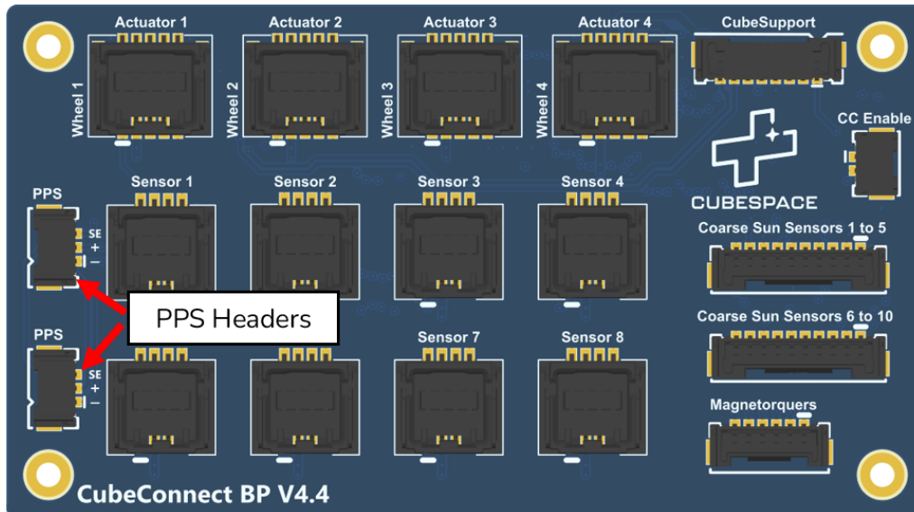
Figure 31: CubeConnect PCB (Backplane Variant) - PPS Headers
