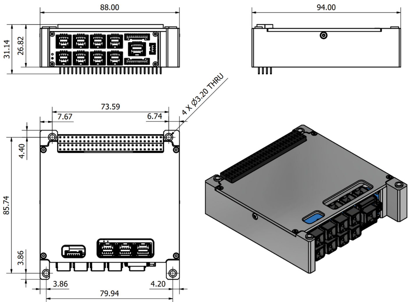
Figure 35: Indicative Dimensions of the Standard PC104 CubeADCS Core
