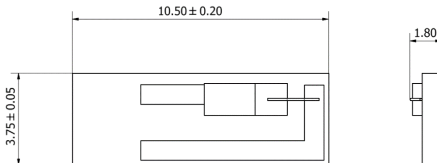
Figure 43: Indicative Dimensions of a Coarse Sun Sensor
