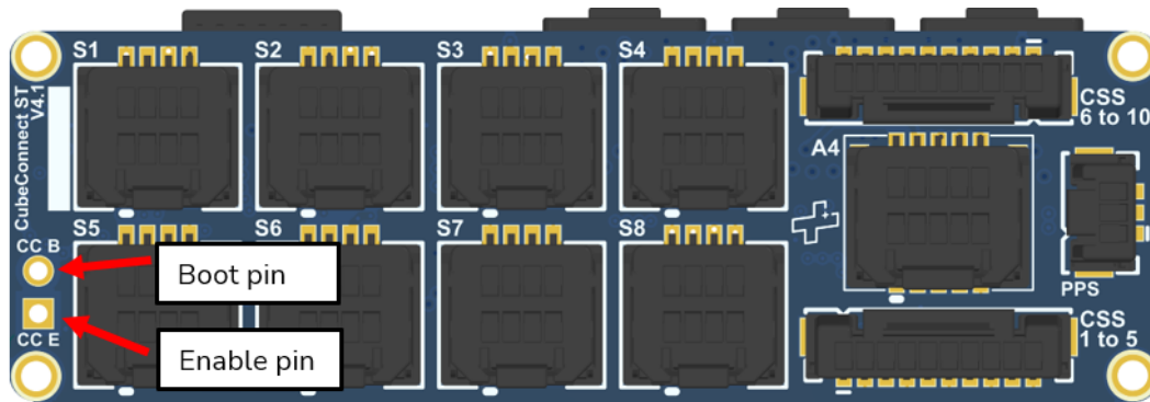
Figure 32: CubeConnect PCB (PC104 Variants) – Additional Boot and Enable Connection Points
