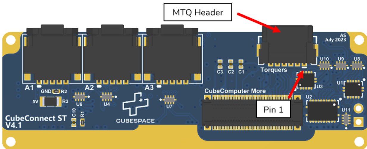
Figure 21: CubeConnect PCB, PC104 Variants (Back View) - Magnetorquer Header
