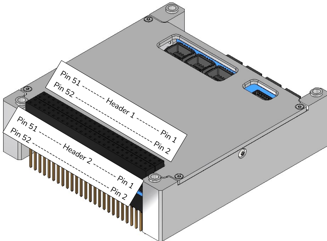
Figure 14: CubeADCS Core, PC104 Variant, Showing CubeDoor Header
